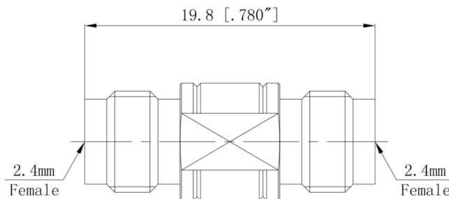
Outline Drawing
